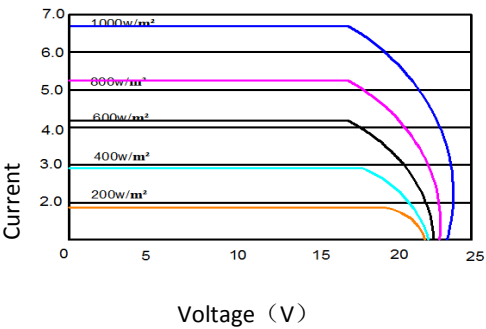
IV-CURVE
