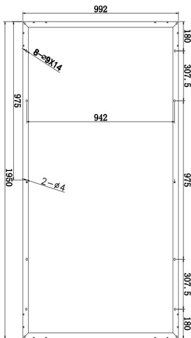
Photovoltaic Module Specification Holes
