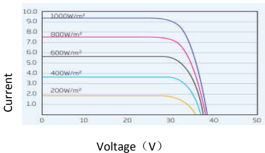
IV-CURVE
