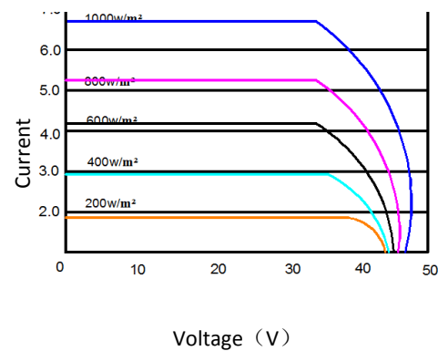
IV-CURVE
