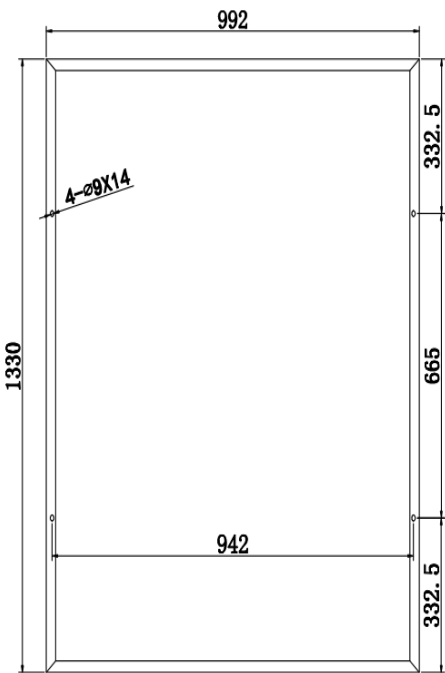
photovoltaic module specification holes
