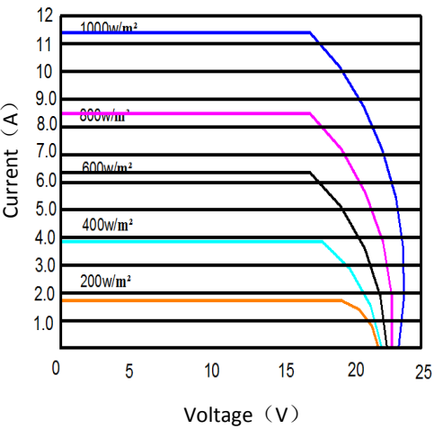
IV-CURVE
